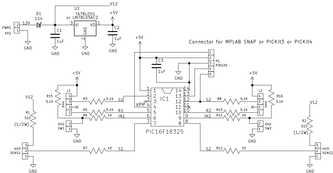
SHUNT_P : Shunting lights control circuit by ik-gadgets
