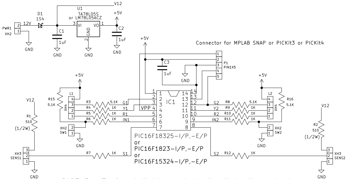
SIG3_P : 3 signal lights control circuit by ik-gadgets
