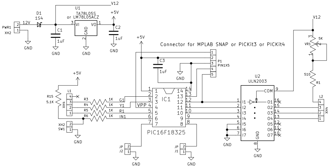
RELAY_P : Relay signal lights control circuit by ik-gadgets
